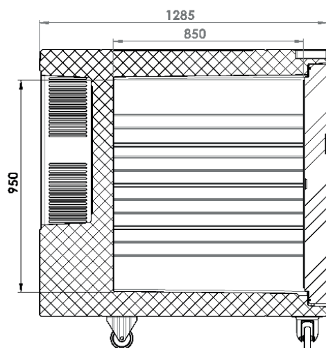
Koala 495 static
