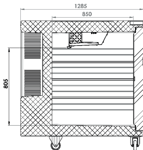
Koala 495 ventilated
