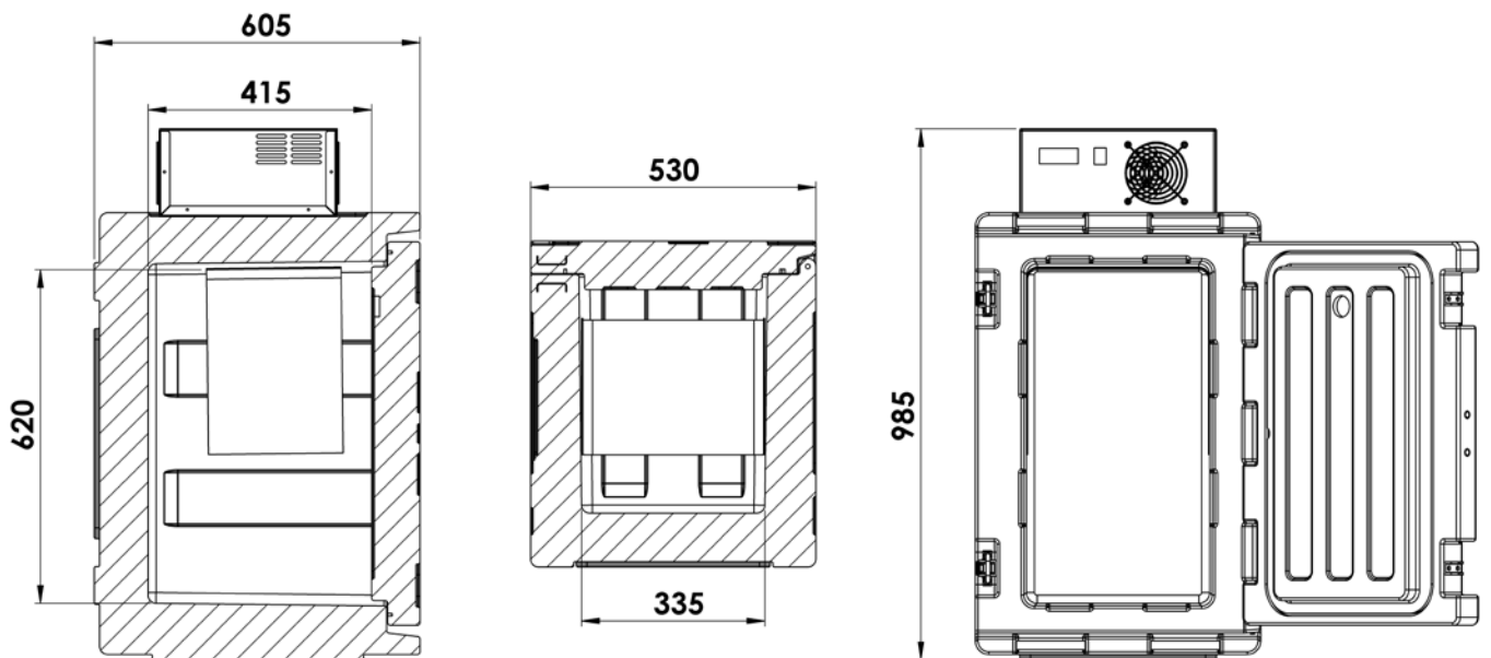
KOALA 90-XTRA TOP COOLING UNIT
