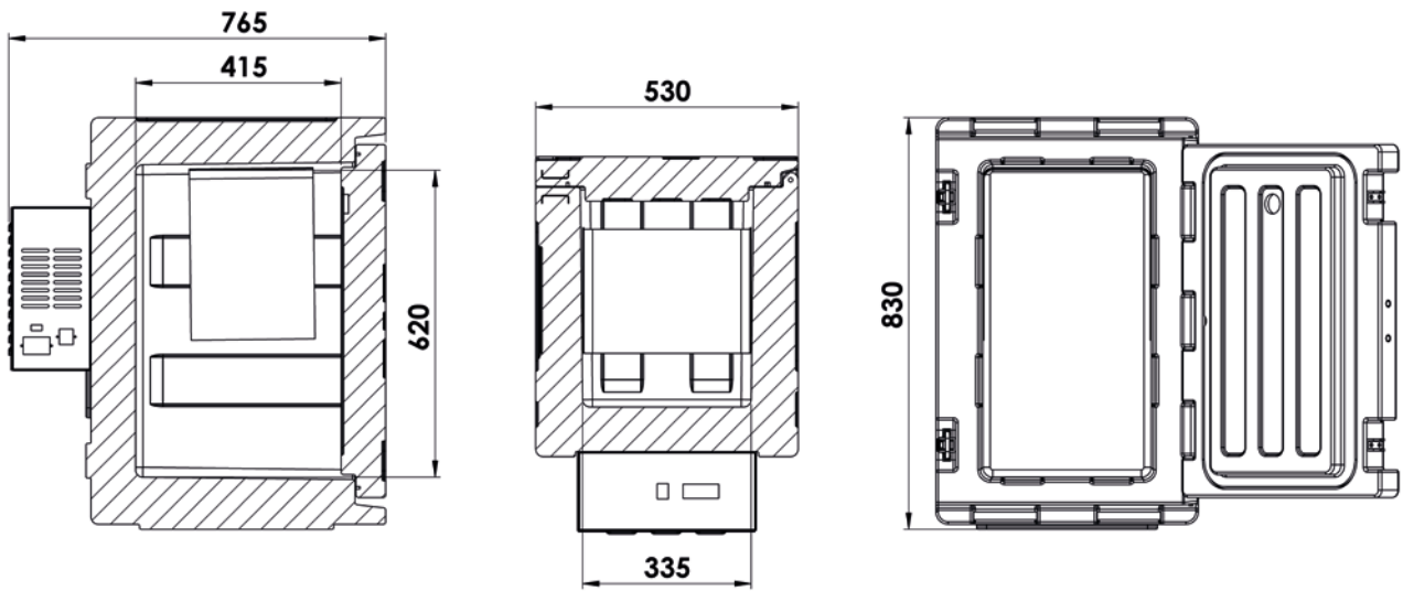
KOALA 90-XTRA BACK COOLING UNIT
